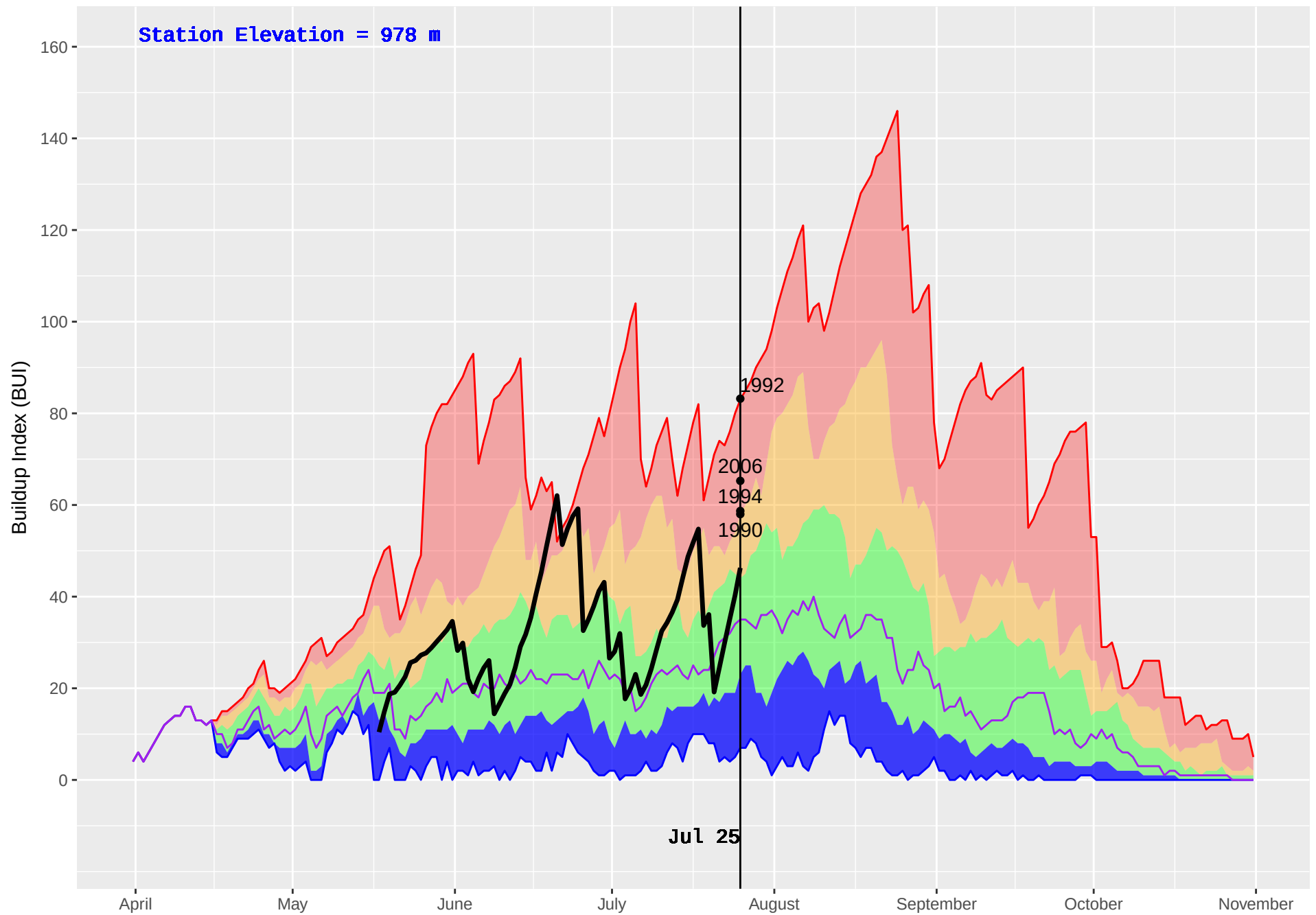
NILKITKWA (172) : Historical (1986–2016) and Current (2018) Noon Buildup Index (BUI)
