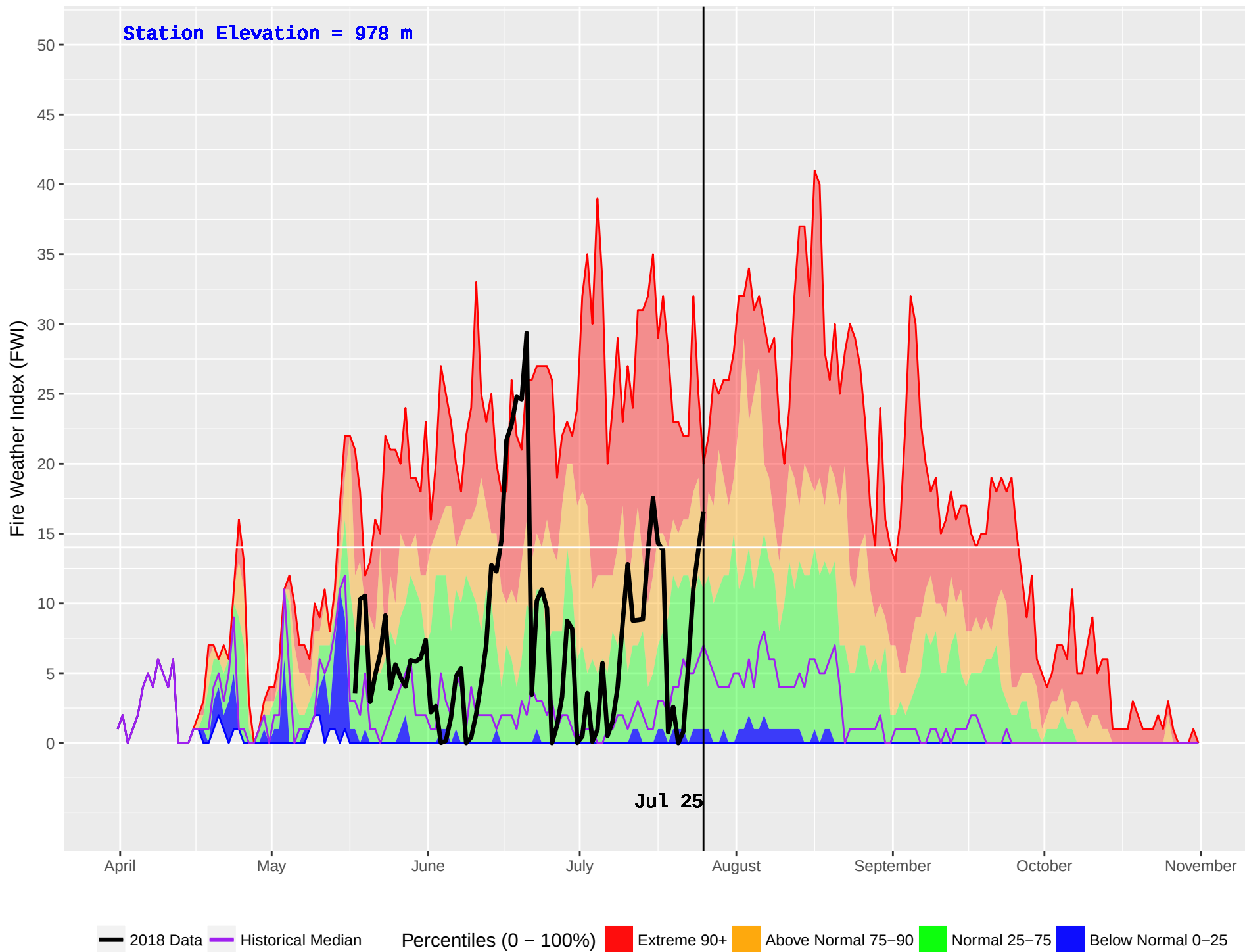
NILKITKWA (172) : Historical (1986–2016) and Current (2018) Noon Fire Weather Index (FWI)
