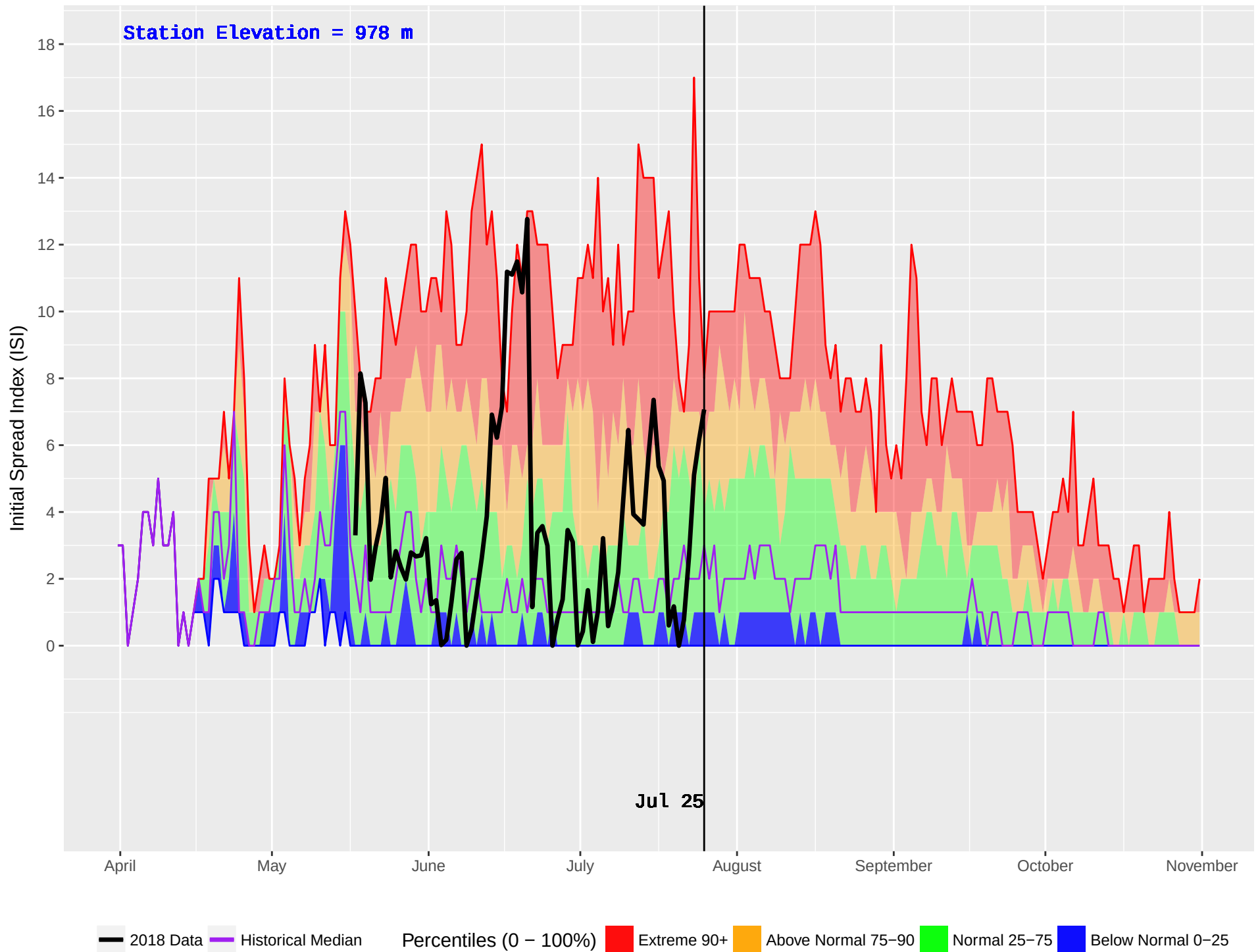
NILKITKWA (172) : Historical (1986–2016) and Current (2018) Noon Initial Spread Index (ISI)
