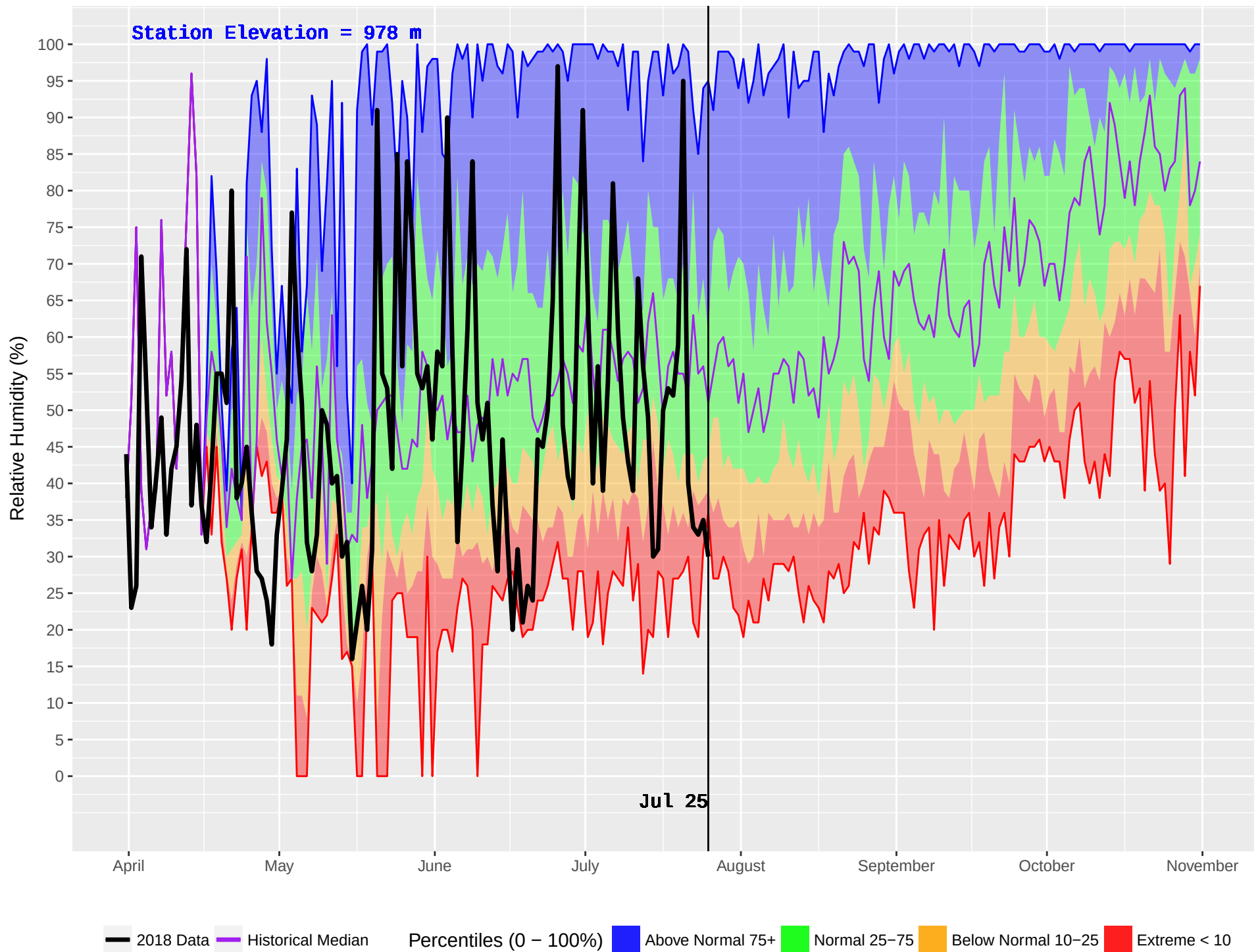
NILKITKWA (172) : Historical (1986–2016) and Current (2018) Noon Relative Humidity
